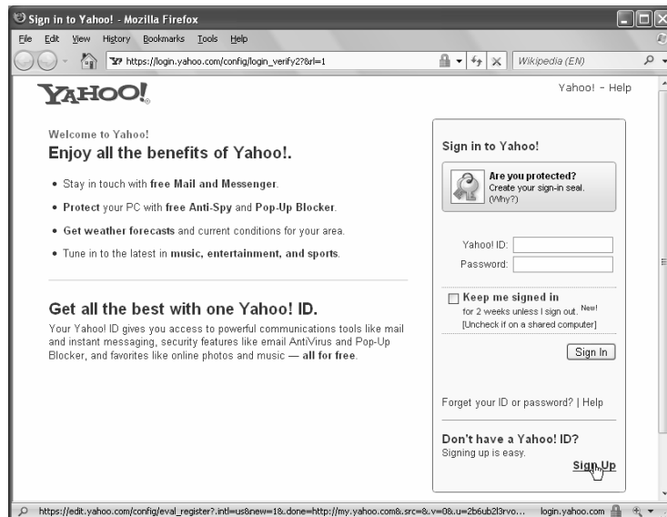
Gambar 1.1 Halaman login.yahoo.com
